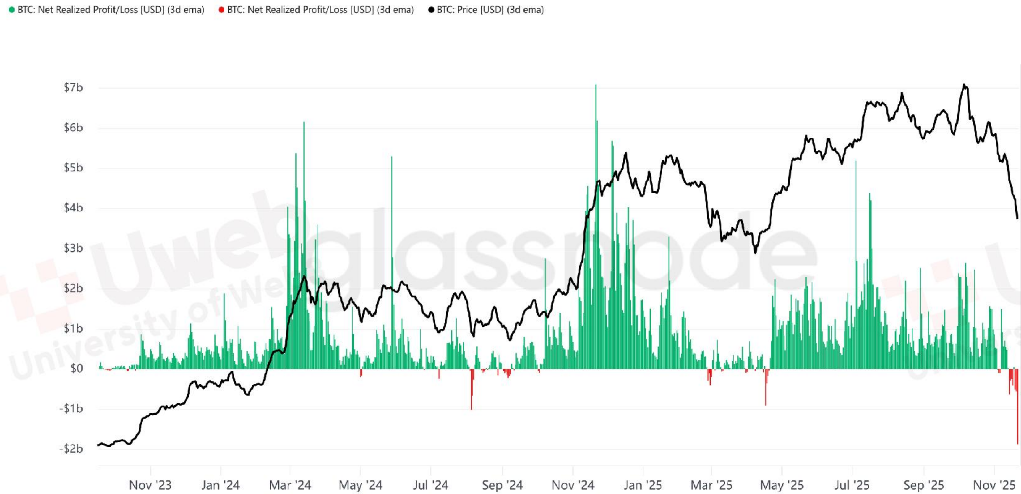
BTC: Net Realized Profit/Loss (3d Exponential Moving Average)
